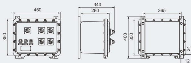
BXM81-4/□/K/□
