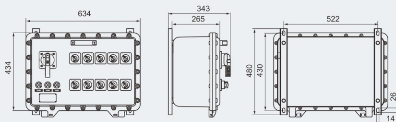
BXM81-10/□/K/□
