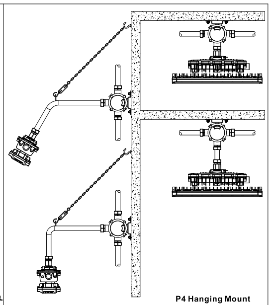
P4 Hanging Mount
