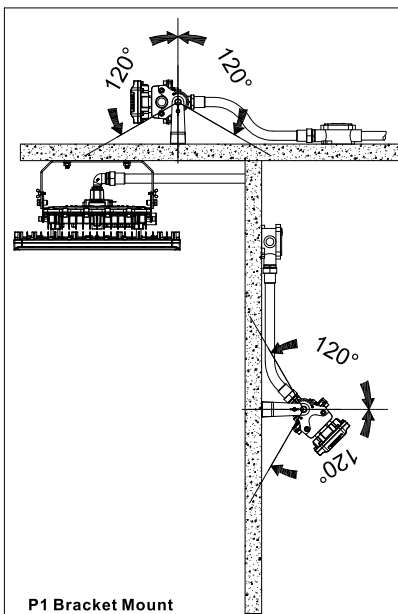
P1 Bracket Mount
