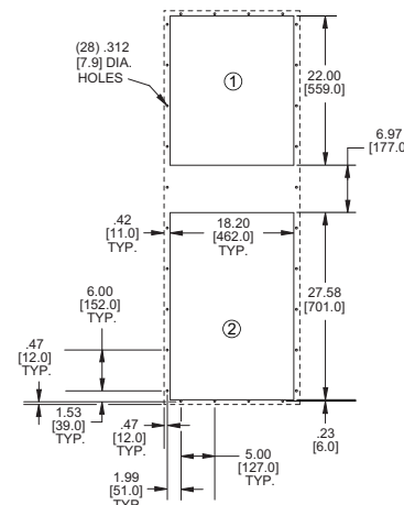
MOUNTING PLAN
