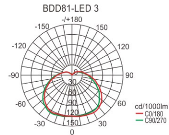
配光曲线 Light distribution curve cd/1000lm
